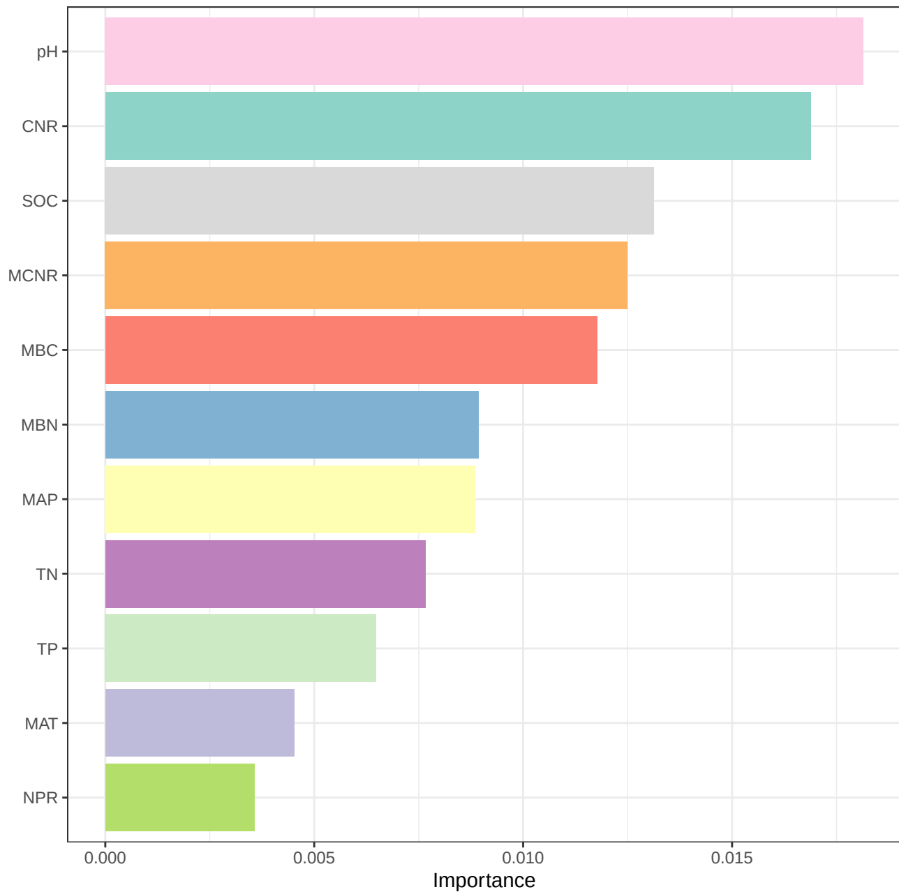
Variable Importance in Final Model
